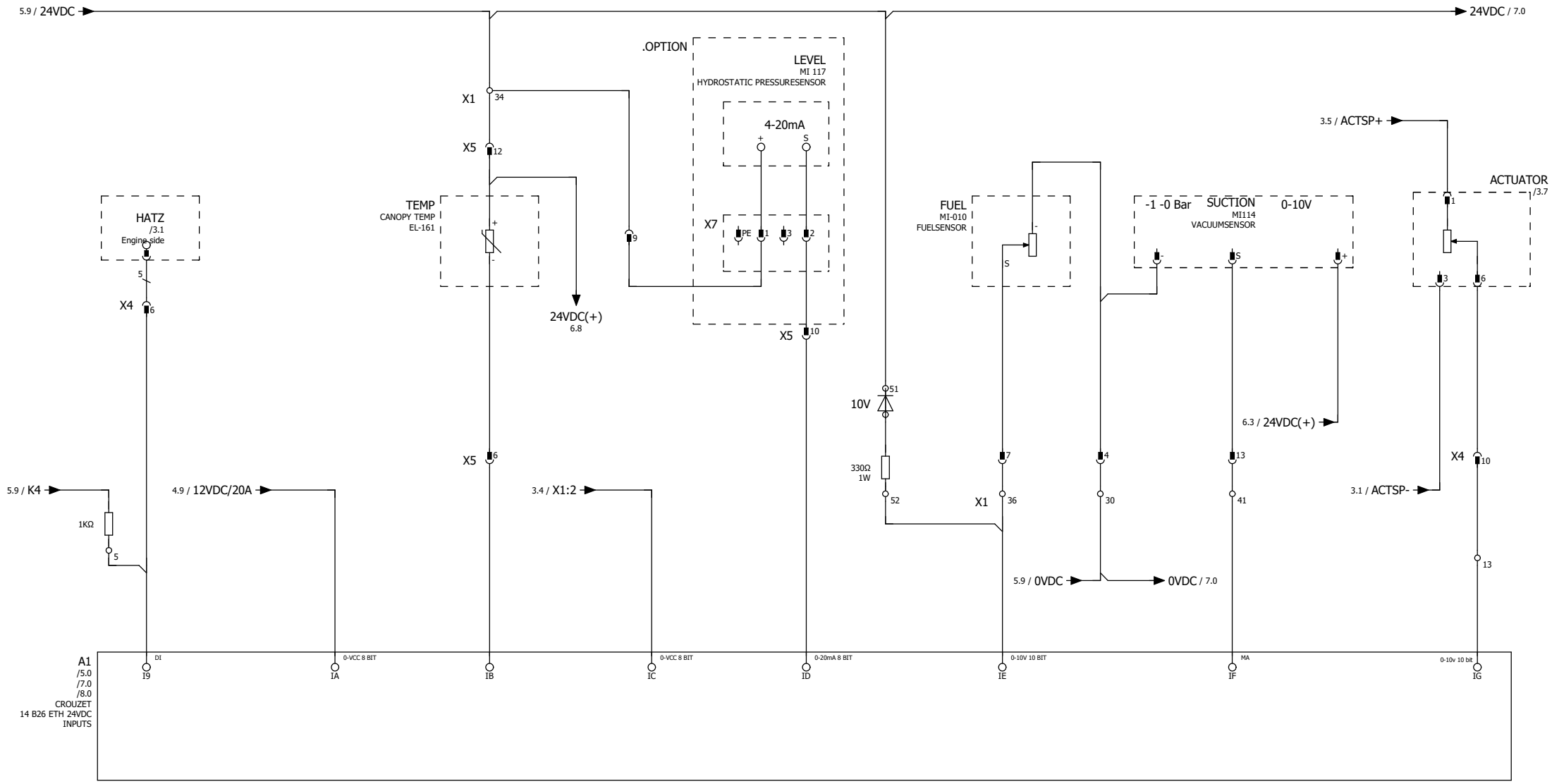
ENGINE TEMP-FAILURE BATTERY VOLTAGE CANOPY TEMP- OPTION DYNAMO VOLTAGE LEVEL SENSOR FUELLEVEL VACUUM SENSOR ACTUATOR FEEDBACK
